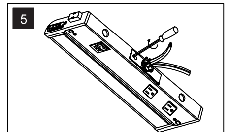
5 Feed wires back in to the fixture, re-attach adapter plate and secure with screws.
