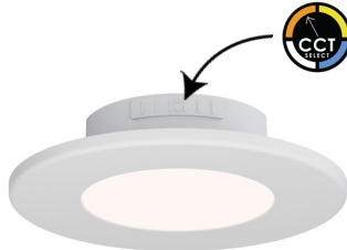
SNUG LED TRIAC OR ELV 87655WTWT 4.75" W x 1" H 11W LED, 27-30-35-40-50 K (800lm) White
